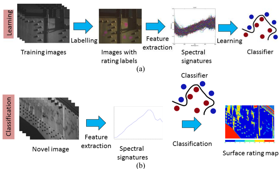
Fig. 3 The process of hyperspectral image analysis for surface condition rating: (a) the (off-line) training phase and (b) in the (online) classification process
